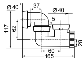
Technical drawing
