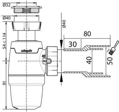
Technical drawing
