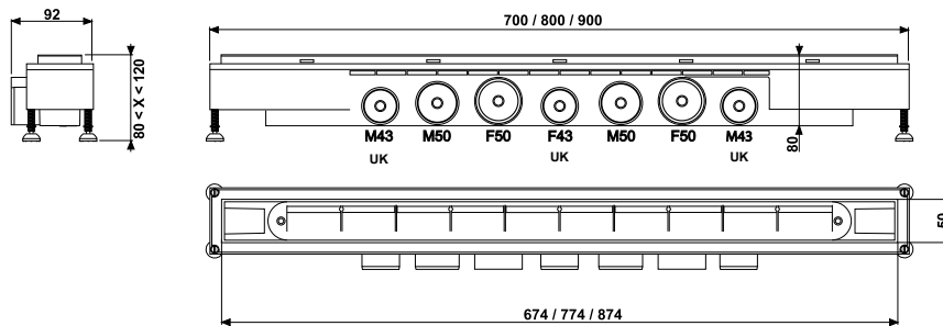
Technical drawing
