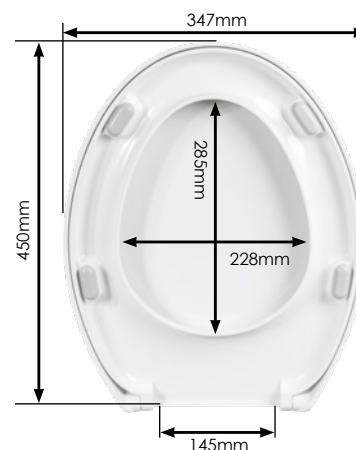
DIAGRAM - 20900002 Full dimensional details per hinge p6
